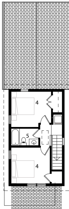
2ND FLOOR PLAN_
