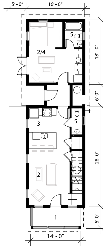
1ST FLOOR PLAN_
