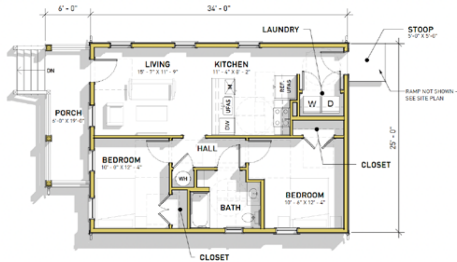
1 FLOOR PLAN SD-2.1 1/8" = 1'-0"
