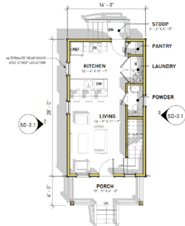
1 FIRST FLOOR PLAN SD-2.1 1/8" = 1'-0"
