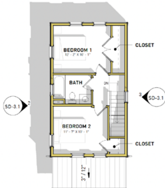
2 SECOND FLOOR PLAN SD-2.1 1/8" = 1'-0"
