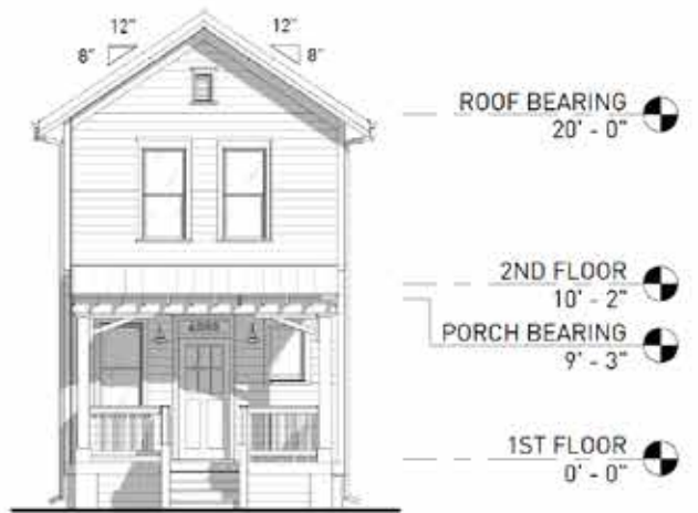
1 FRONT ELEVATION SD-3.1 1/8" = 1'-0"
